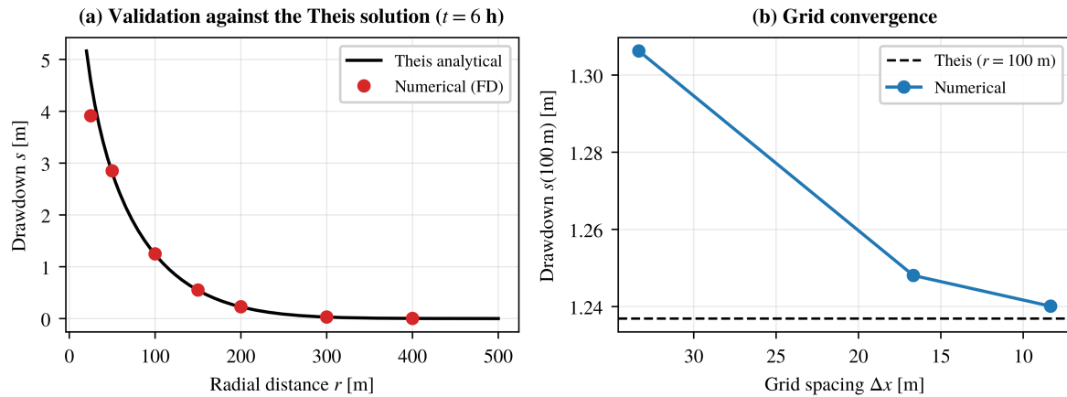
Figure 4. Verification and validation: (a) computed transient drawdown (points) against the Theis analytical solution (line) at t = 6 h for a single well in a homogeneous confined aquifer; (b) grid convergence of the drawdown at r = 100 m toward the analytical value as \Delta x \rightarrow 0 .
