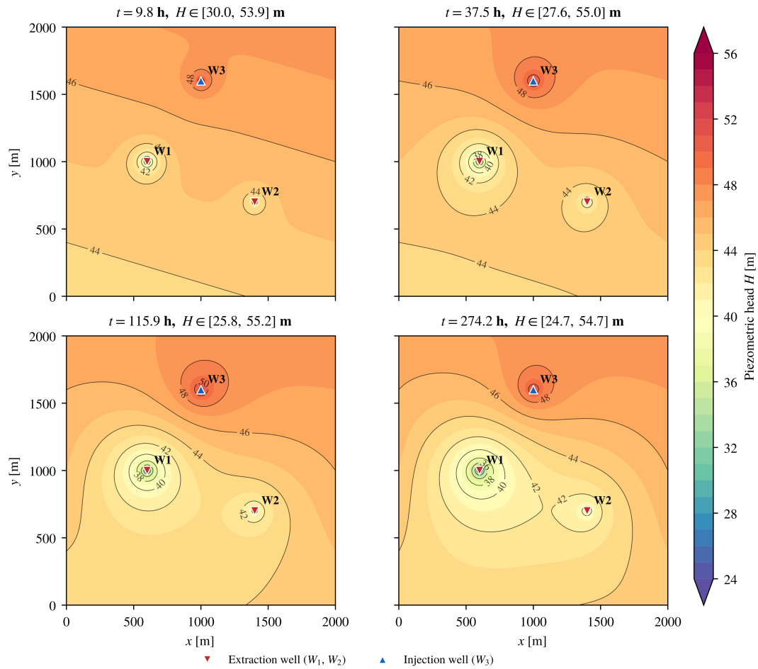
Figure 1. Evolution of the piezometric head H(x, y) at t = 9.8, 37.5, 115.9 and 274.2 h. Red triangles are the extraction wells W_1, W_2 ; the blue triangle is the injection well W_3 . The colour scale is common to all four panels.
