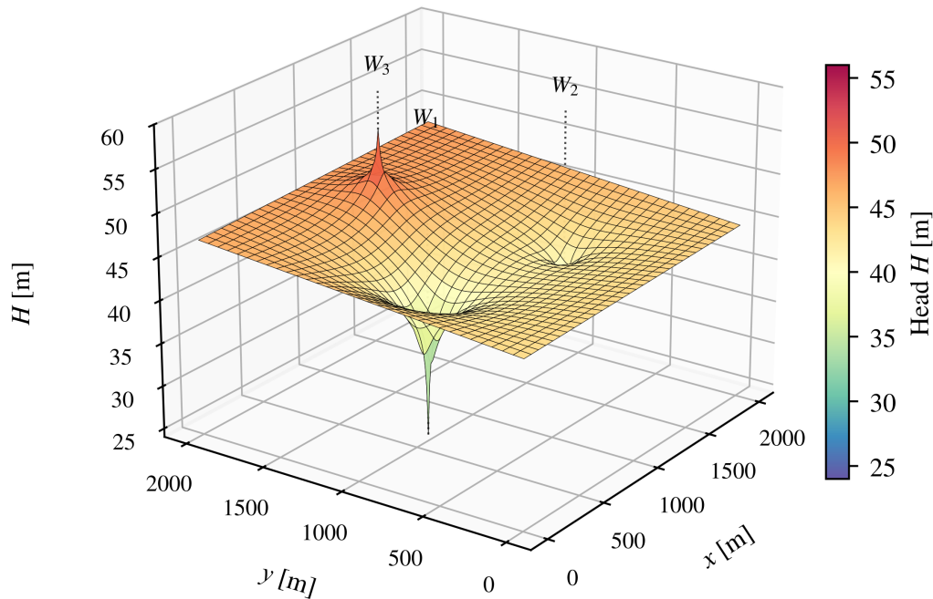
Figure 3. Three-dimensional view of the head surface at t = 274.2 h. The two funnels are the extraction cones ( W_1 , W_2 ) and the peak is the injection mound ( W_3 ), superimposed on the inclined regional surface.
