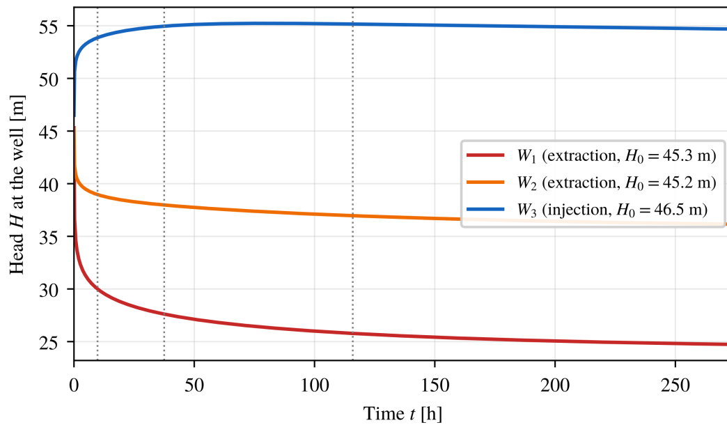
Figure 2. Transient head response at the three wells. The extraction wells W_1, W_2 draw down while the injection well W_3 builds up; dotted lines mark the four snapshot times of Fig. 1.
